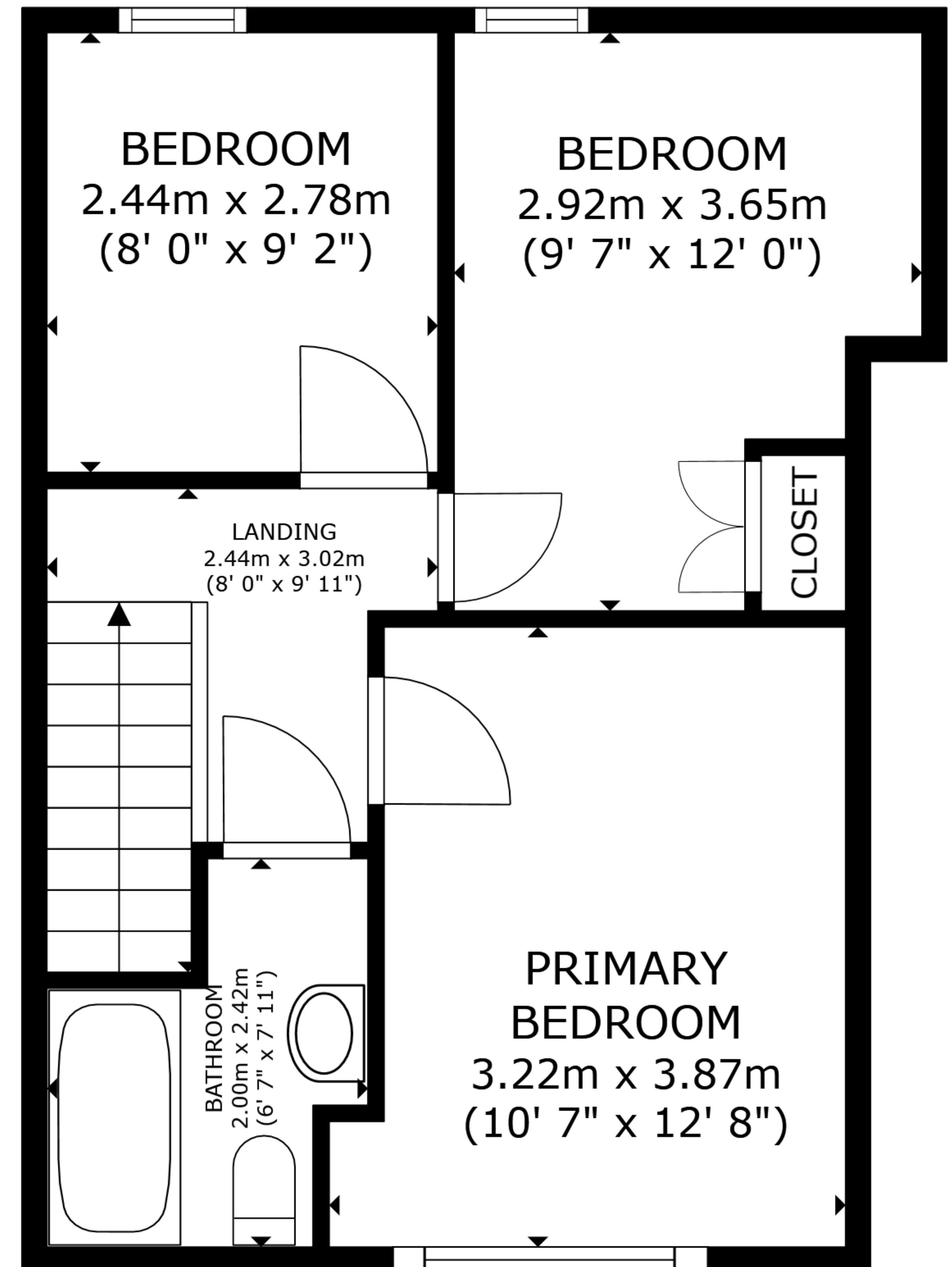
FLOOR 2
